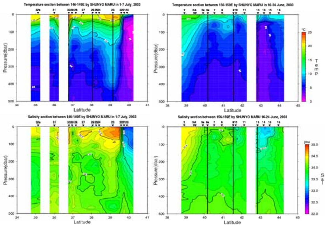
Fig. 6. Temperature (upper panels) and salinity (lower panels) between 146° E-149° E (left panels) and between 156° E-159° E (right panels) observed by R/V Shunyo Maru in 16-24 June and 1-7 July 2003.
