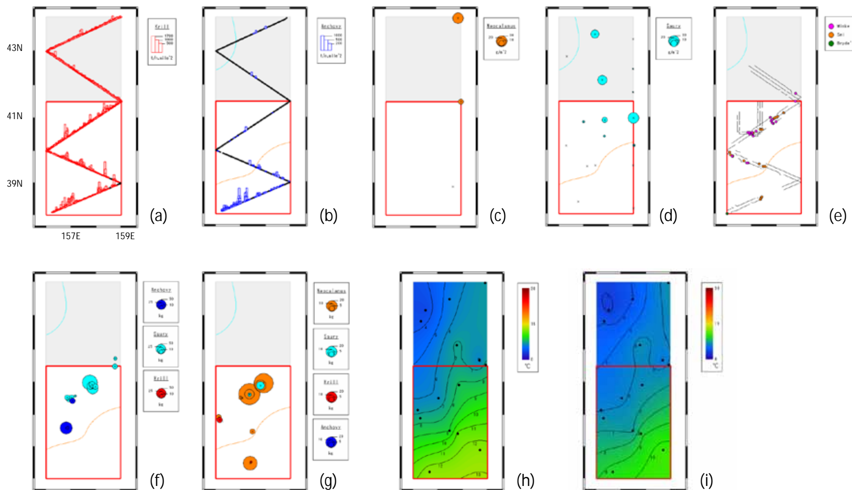
Fig.4. Maps in block A in 2003: Distribution patterns of krill (a), Japanese anchovy (b), copepods ( Neocalanus spp. (C5)) (c) and Pacific surary (d). Sighting effort and sighting positions of common minke and sei whales (e). Sampled positions and stomach contents of minke (f) and sei (g) whales. Water temperature at 100 m (h) and 200 m (i) water depth. Encircled area by red line is the poststratified area, A-S. Light blue and orange lines in maps (a)-(g) represent 4°C and 10°C isotherm at 100 m water depth, respectively.
