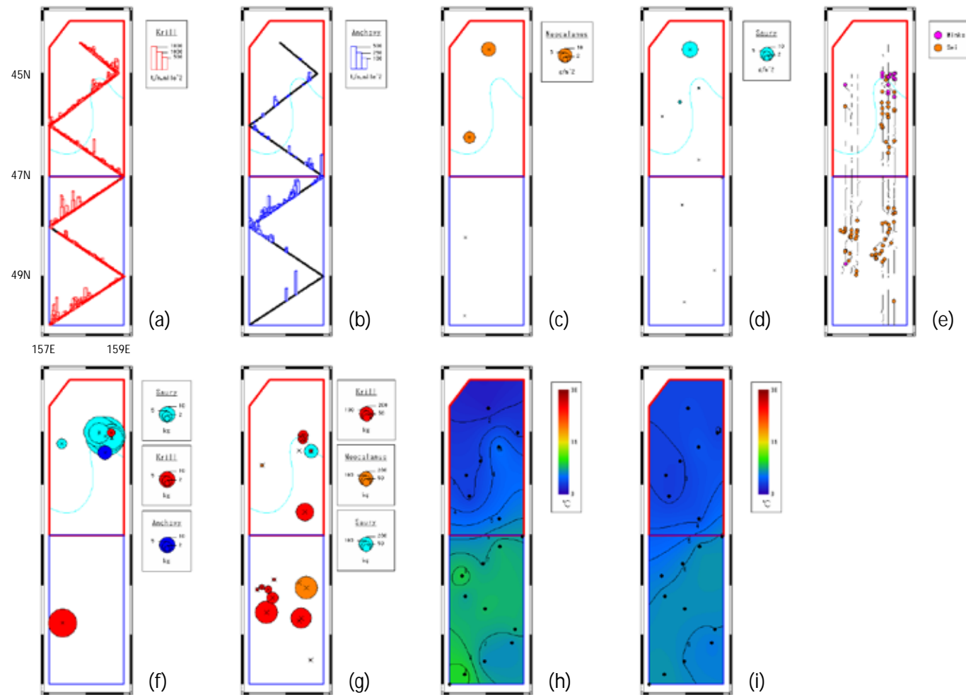
Fig.7. Maps in block E in 2005: Distribution patterns of krill (a), Japanese anchovy (b), copepods ( Neocalanus spp. (C5)) (c) and Pacific suary (d). Sighting effort and sighting positions of common minke and sei whales (e). Sampled positions and stomach contents of minke (f) and sei (g) whales. Water temperature at 100 m (h) and 200 m (i) water depth. Encircled areas by red and blue lines are the poststratified area, E-N and E-S, respectively. Light blue line in maps (a)-(g) represents 4°C isotherm at 100 m water depth.
