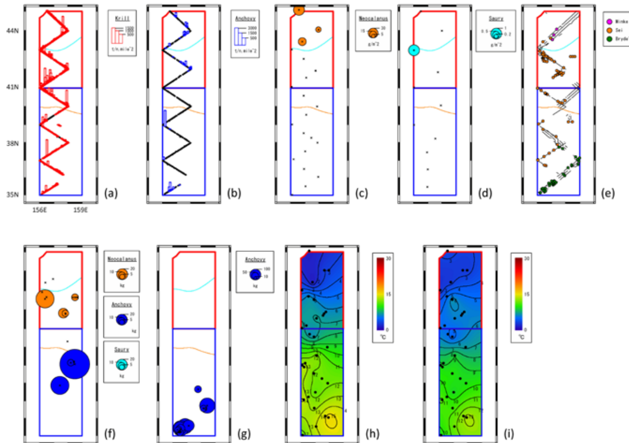
Fig.9. Maps in block 1 in 2007: Distribution patterns of krill (a), Japanese anchovy (b), copepods ( Neocalanus spp. (C5)) (c) and Pacific suary (d). Sighting effort and sighting positions of common minke Bryde's and sei whales (e). Sampled positions and stomach contents of minke (f) and sei (g) whales. Water temperature at 100 m (h) and 200 m (i) water depth. Encircled areas by red blue lines are the poststartified area, E-N and E-S, respectively. light blue and orange lines in maps (a)-(g) represent 4°C and 10°C isotherm at 100 m water depth, respectively.
