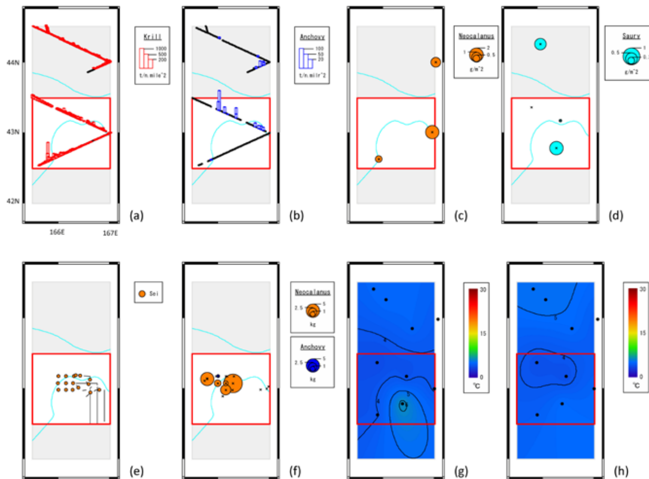
Fig.6. Maps in block O in 2004: Distribution patterns of krill (a), Japanese anchovy (b), copepods ( Neocalanus spp. (C5)) (c) and Pacific surary (d). Sighting effort and sighting positions of sei whales (e). Sampled positions and stomach contents of sei whales (f). Water temperature at 100 m (g) and 200 m (h) water depth. Encircled area by red line is the poststratified area, O-C. Light blue and line in maps (a)-(f) represents 4°C isotherm at 100 m water depth.
